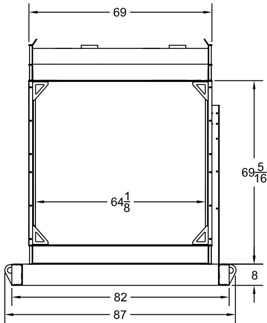
RADIATOR VIEW
