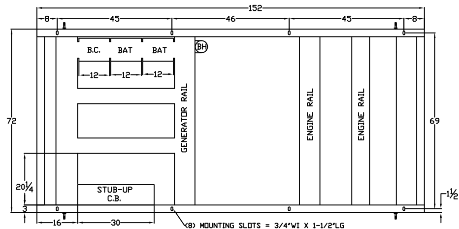
FRAME VIEW
