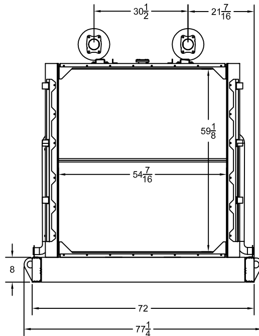
RADIATOR VIEW
