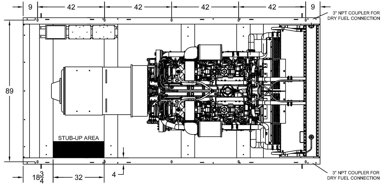
TOP VIEW
