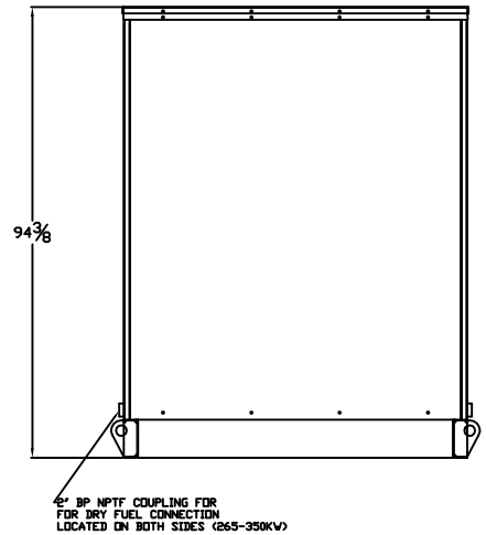
RADIATOR END VIEW
