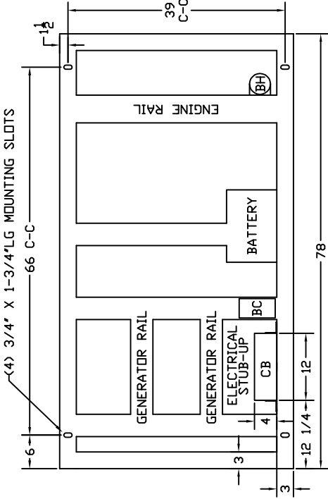
FRAME VIEW
