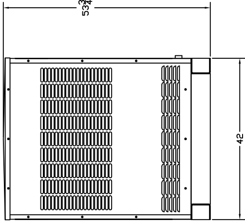
GENERATOR END VIEW
