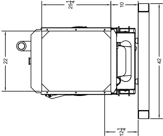
RADIATOR VIEW
