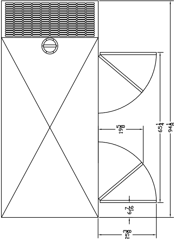
TOP VIEW
