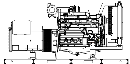
“OPEN” GEN-SET
