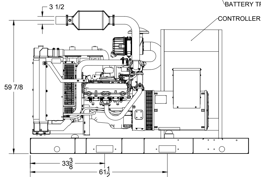
SIDE VIEW
