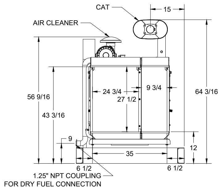
RADIATOR VIEW
