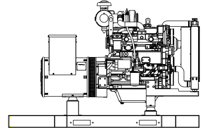
"OPEN" GEN-SET
