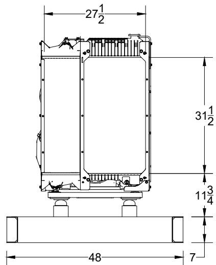
RADIATOR VIEW
