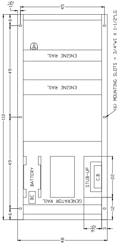
FRAME VIEW
