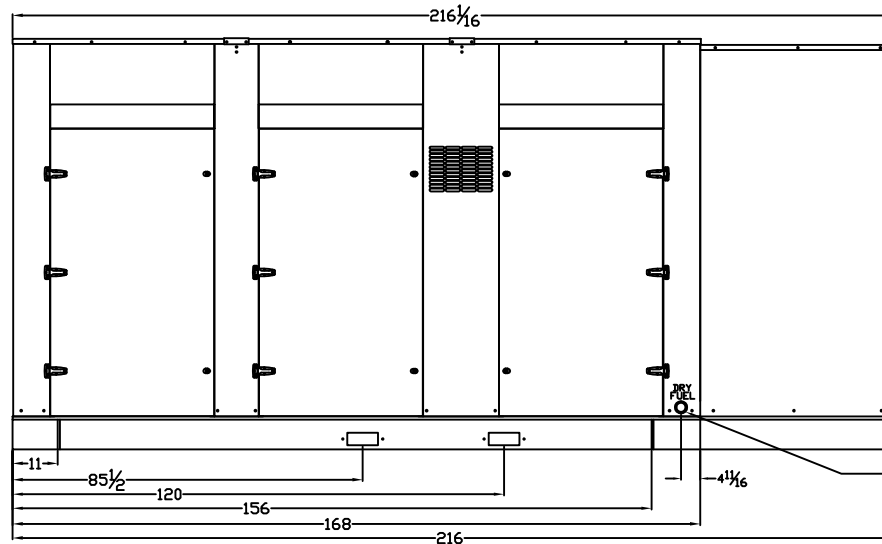
SIDE VIEW
