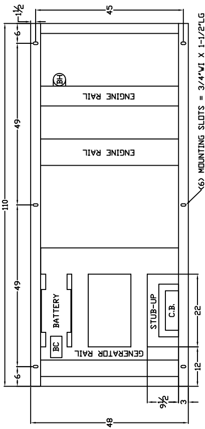
FRAME VIEW
