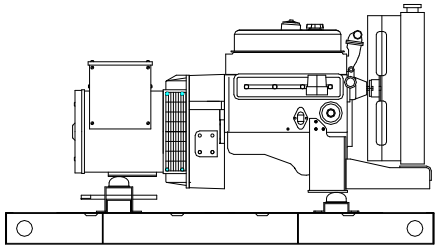
“OPEN” GEN-SET
