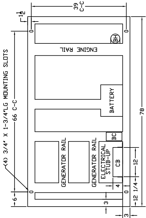
FRAME VIEW
