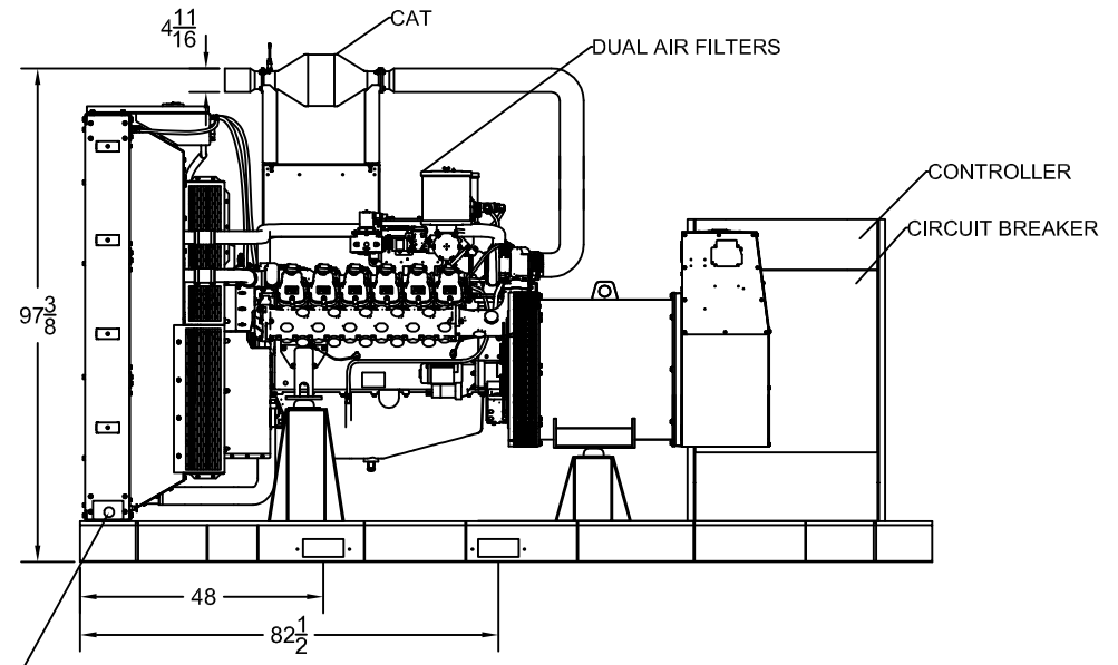
SIDE VIEW
