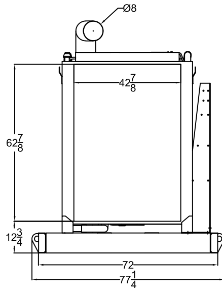
RADIATOR VIEW
